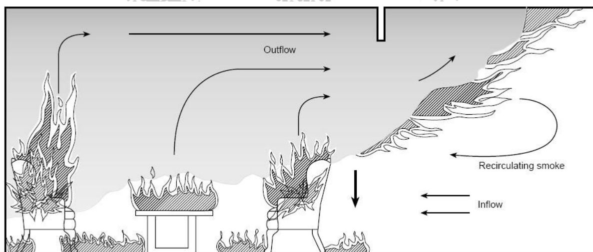
Flashover conditions in compartment fire.
