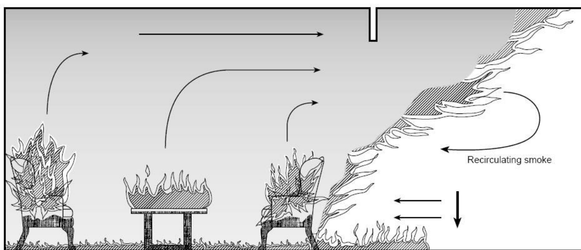
Postflashover or full room involvement in compartment fire.
