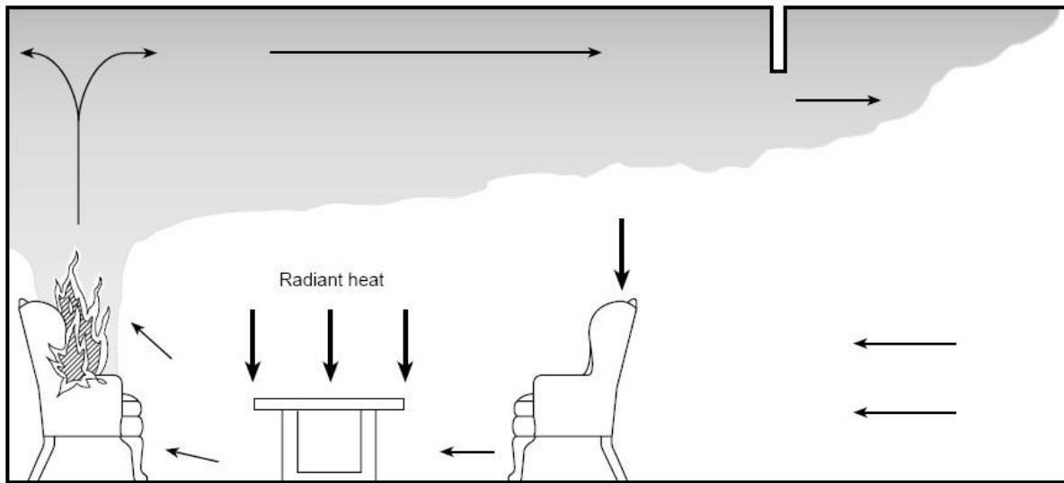
Preflashover conditions in compartment fire.
